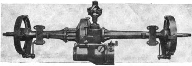
Individuality In Autocar Rear Construction.
